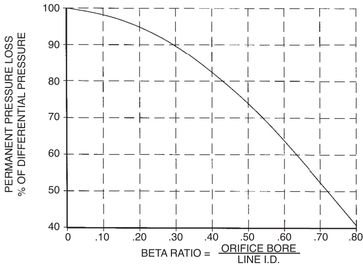
PERMANENT PRESSURE DROP VS BETA RATIO FOR ORIFICE PLATE WITH FLANGE TAPS
