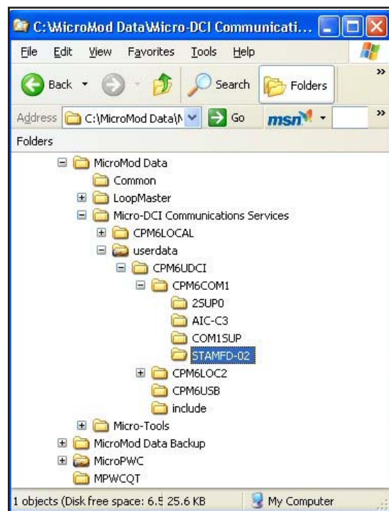
Figure 5 Controller folders
